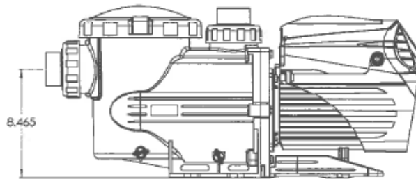
(Figure 3a) Pump shown without universal base
